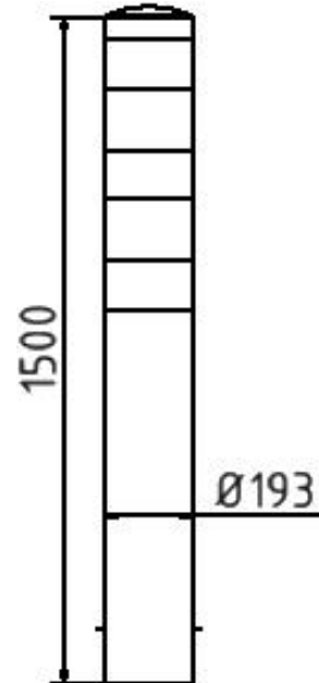
Impact protection bollard Ø 193 mm
