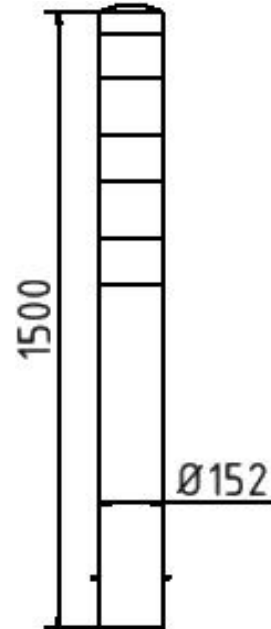
Impact protection bollard Ø 152 mm
