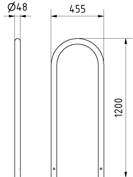
Barrier bracket Ø 48 mm
