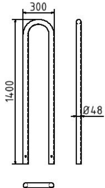
Barrier bracket Ø 48 mm
