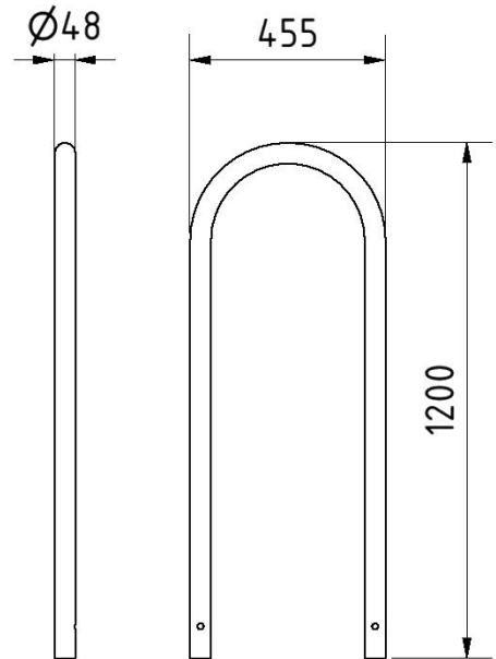
Barrier bracket Ø 48 mm
