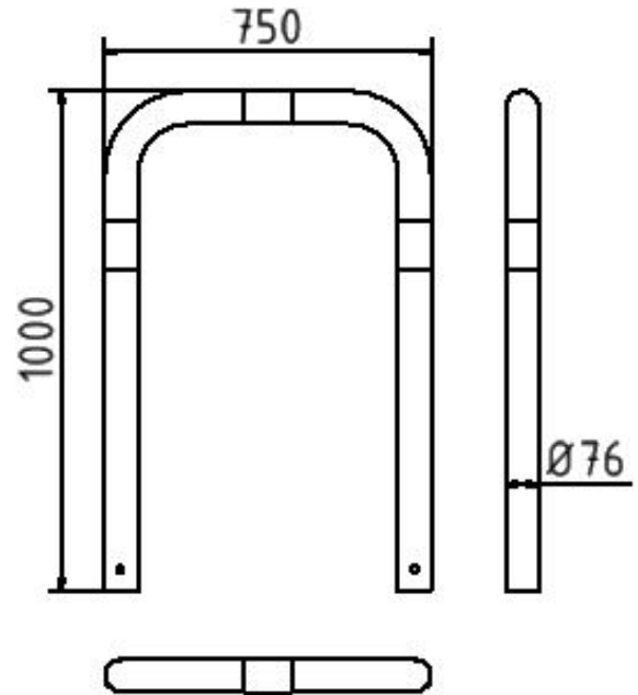
Impact protection bracket Ø 76 mm
