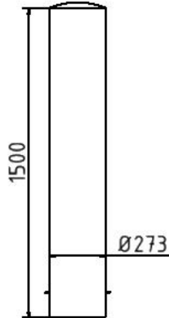
Steel tube bollard Ø 273 x 5 mm
