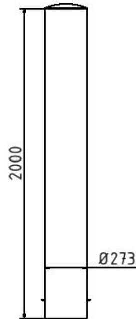
Steel tube bollard Ø 273 x 5 mm
