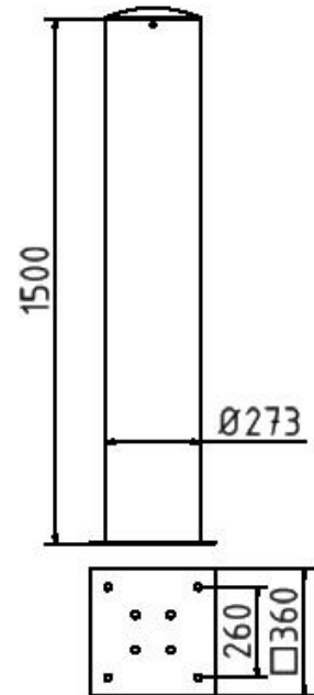
Steel tube bollard Ø 273 x 5 mm
