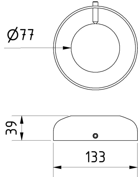
Ground rosette for post, Ø 76 mm
