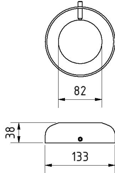
Ground rosette for post, Ø 82 mm
