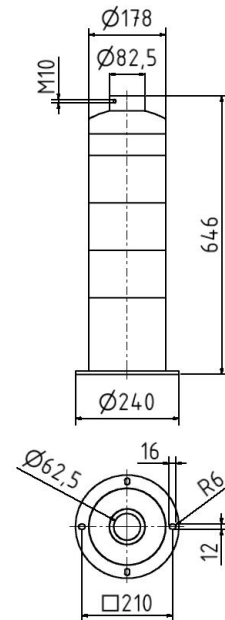
Island post type 44170BG -stationary-
