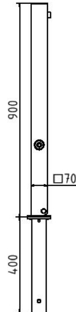
Stainless steel post 70 x 70 mm, without eyelet
