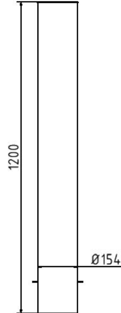
Stainless steel post Ø 154 mm
