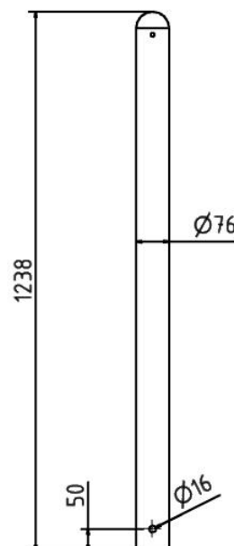
Barrier post type 4077B
